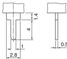
Printed circuit Terminal
